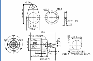
TRB JACK RECEPT BULKHEAD STRAIGHT
